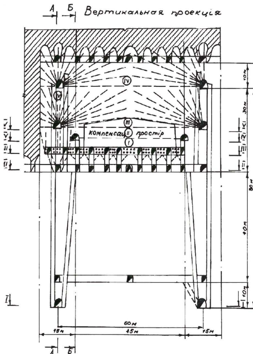
Fig. 1. A variant of the room-and-pillar system with formation of a vaulted crown: I, II, III, IV - stages of forming a vaulted crown of a stope
