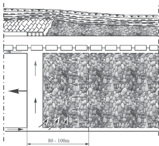
Fig. 2 Methane migration through goafs
