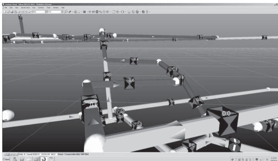
Fig. 8 Simulation of \text{CO}_2 dispersion at ventilation network level
