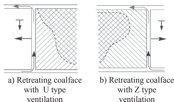
Fig. 1 Coalface advancing and ventilation manner
