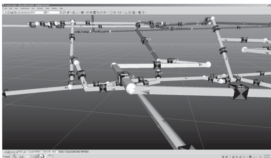
Fig. 9 Simulation of \text{CO} dispersion at ventilation network level
