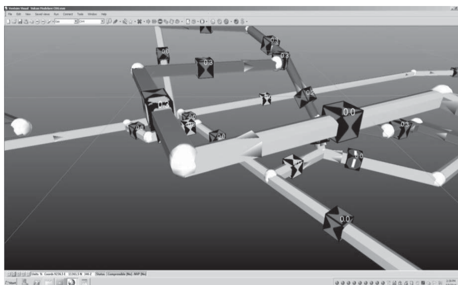
Fig. 4 Simulation of \text{CH}_4 dispersion at ventilation network level
