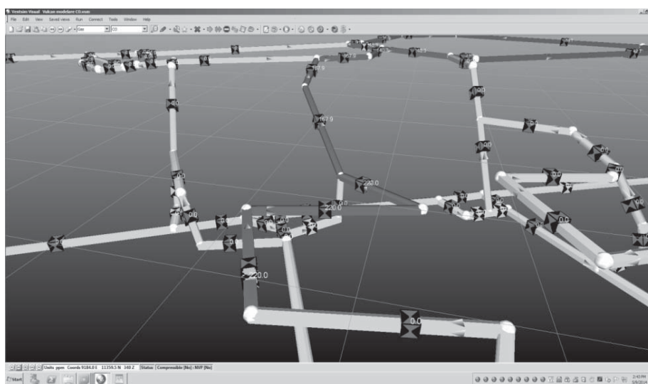
Fig. 6 Simulation of CO dispersion at ventilation network level
