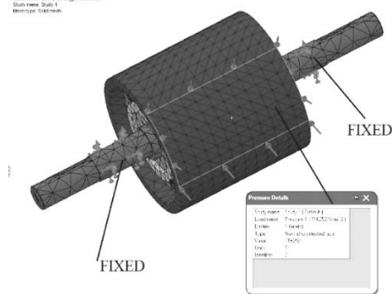
Fig. 7 Boundary conditions imposed on the model and its discretisation (netting) within the Cosmos Works medium
