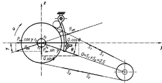
Fig. 3 Forces in the belt gearing drive
