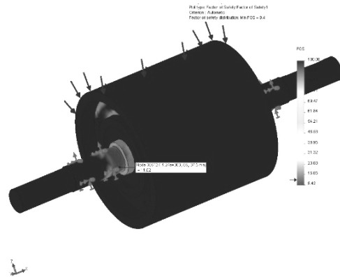
Fig. 9 Distribution of the safety factor (FOS) over the drive shaft and the rotor of the crusher
