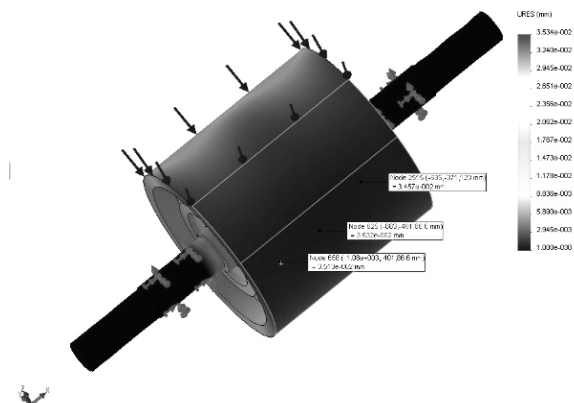
Fig. 10 Distribution of the static displacement of the shaft and rotor
