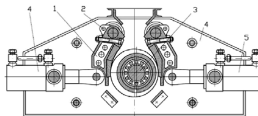
Fig. 1 Rotary crusher
