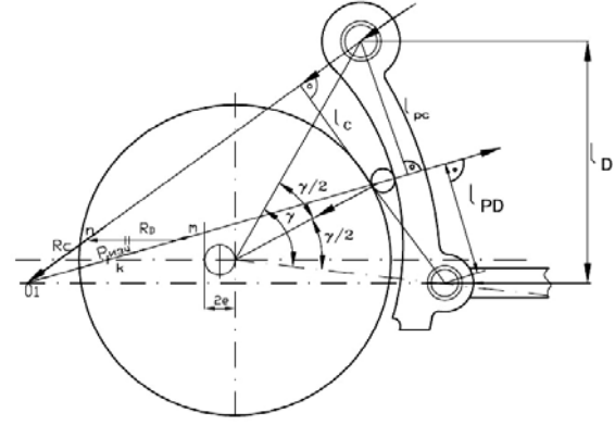
Fig. 2 Crushing force and support reactions
