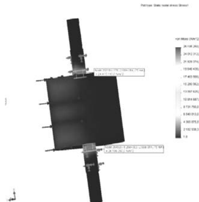
Fig. 8 Distribution of the equivalent stresses on the CAD-CAE model
