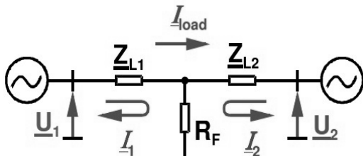
Fig.1 Simple model for the effect of fault resistance at double-ended infeed (load flow from left to right)
