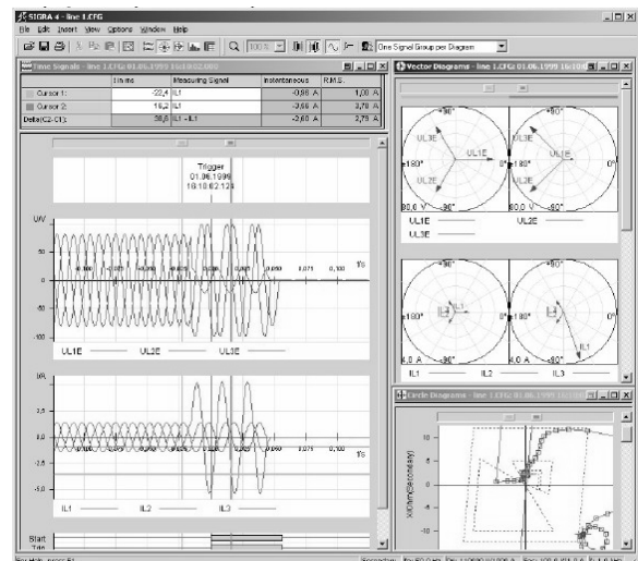
Fig.3 Fault oscillogram, phasor diagram and impedance locus derived from one fault record
