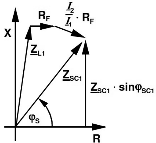
Fig.2 Double infeed fault resistance affecting the measured reactance
