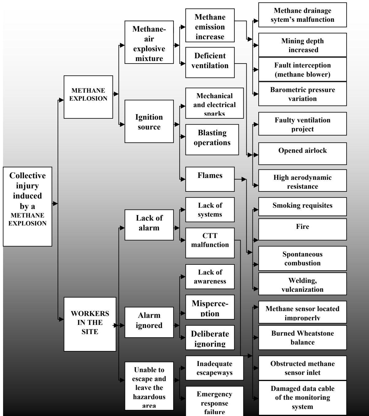
Figure 1 Reduced Tree – Cause tree for the undesired event „Collective injury induced by a methane explosion“
